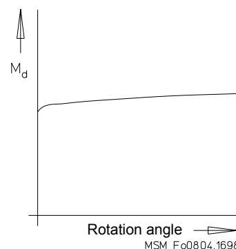
Fig. 3: Torque characteristic
