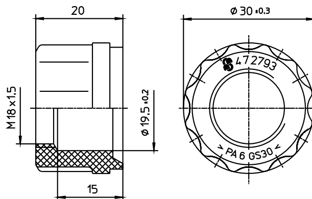
Fig. 6: Fastening nut 472793 Suitable socket wrench SW26 (12 bihex DIN 3124) O-ring to be used: 19 x 2,5 70 shore A Tightening torque 5 +1 Nm
