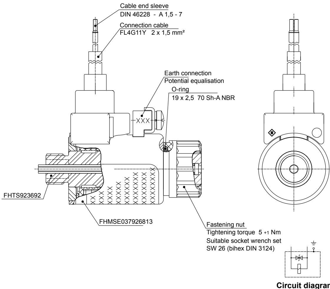
Fig. 5: Proportional solenoid G HP E 037 A GD A01
