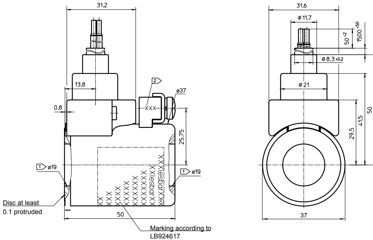
Fig. 3: Magnetic body 924617 (FHMSE037924617)
